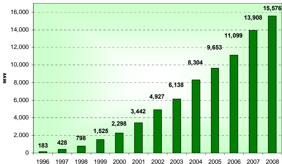
Installed Wind power generation evolution 1996-2008
