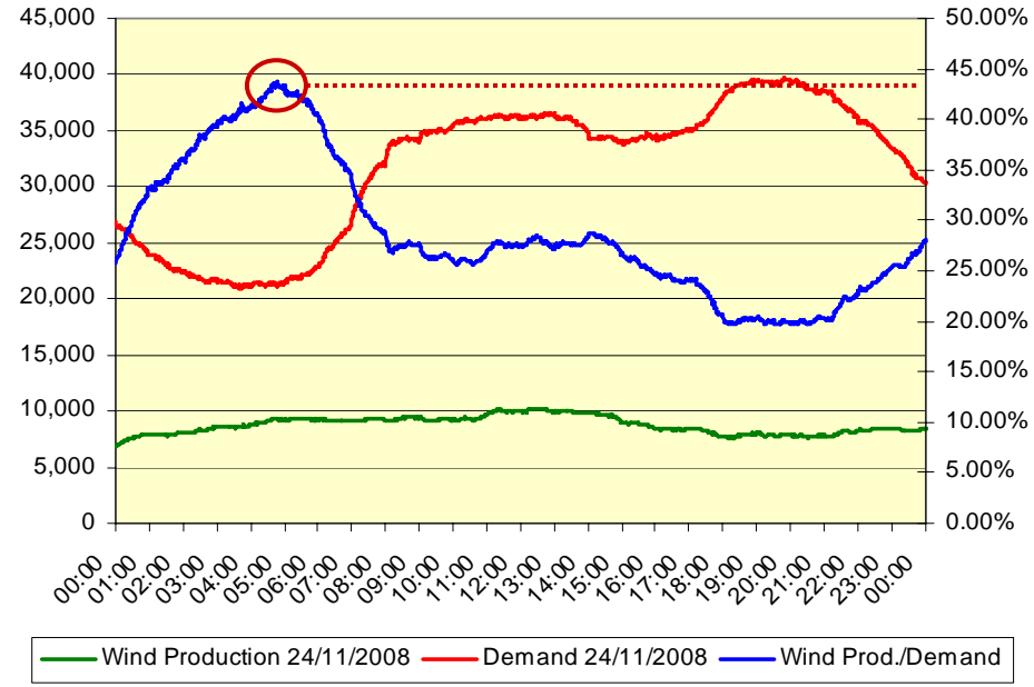
DEMAND vs. WIND PRODUCTION
